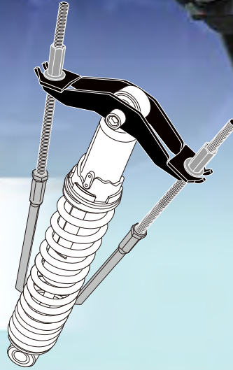
Bolt Spring hook Spring compressor Body
