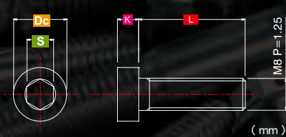
Caliper Bridge Bolt (mm)
